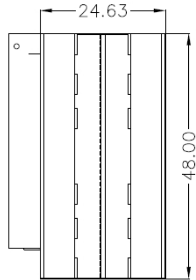
TOP VIEW (SHOWN LESS GRATE)
