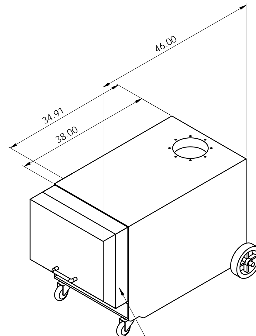
EXTERNAL HEPA/SILENCER OPTION (CAN BE ROTATED 180° FOR UPWARD EXHAUST)
