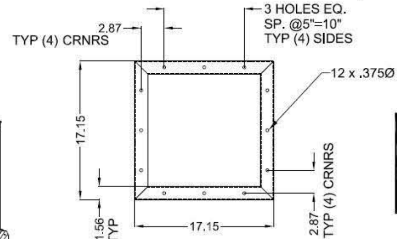
HOPPER OUTLET
