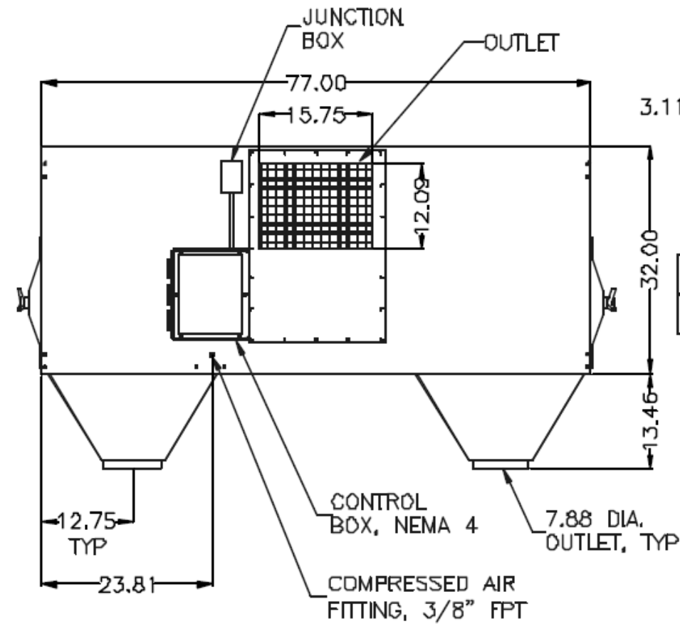
SIDE VIEW
