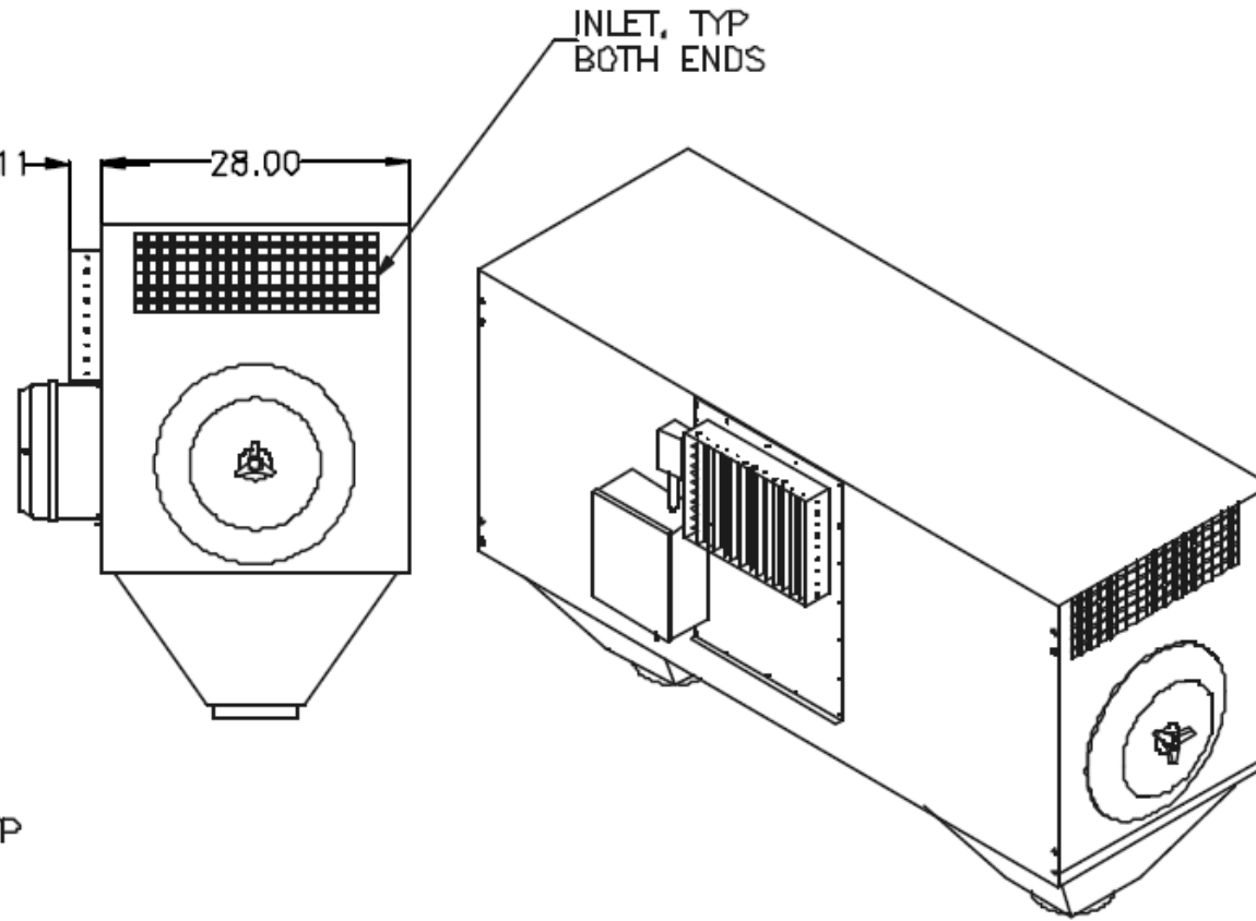
END VIEW
